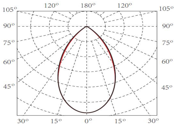
灯具配光曲线 Light distribution curve
