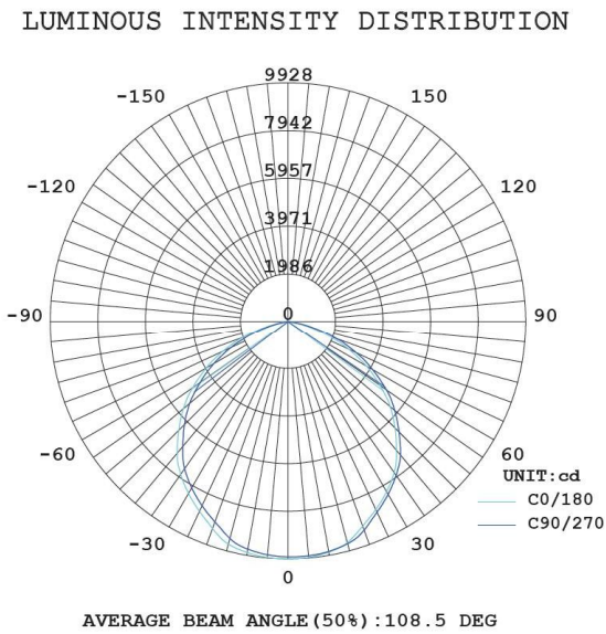
灯具配光曲线 Light distribution curve
