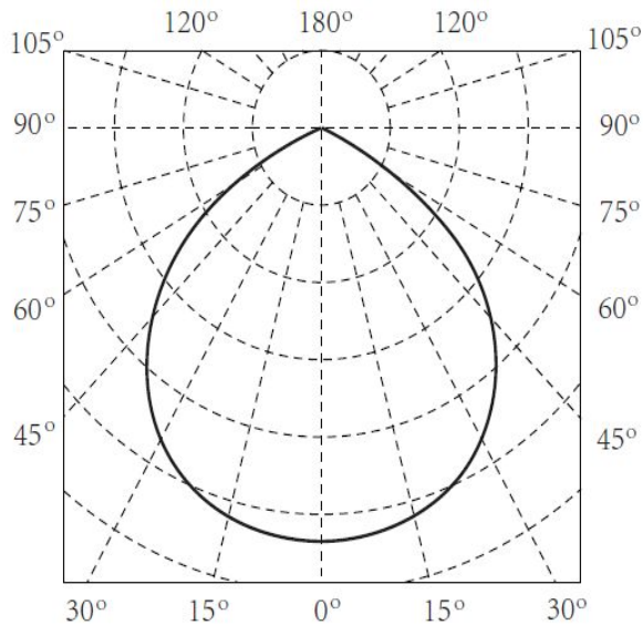
灯具配光曲线 Light distribution curve
